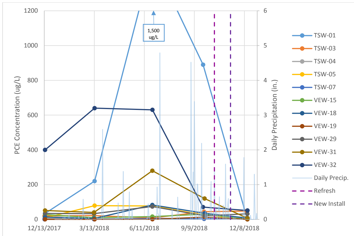
Figure 3.2 UGR Well PCE Concentration Trends
