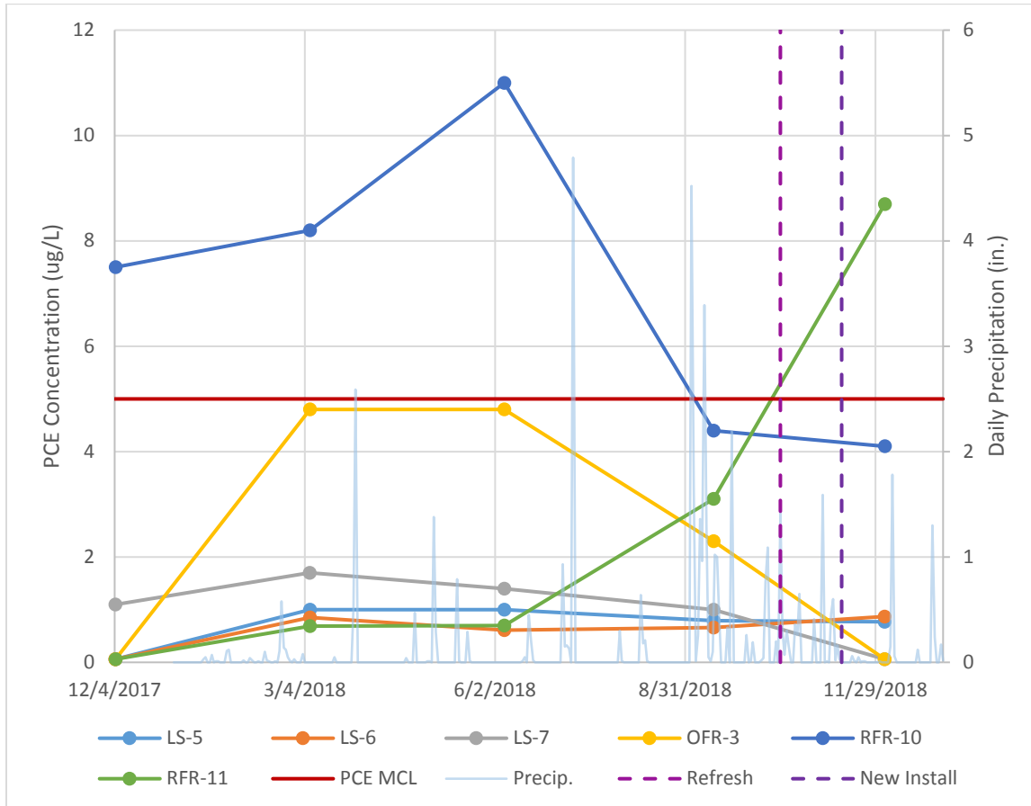
Figure 3.3 Off-Post Supply Well PCE Concentration Trends
