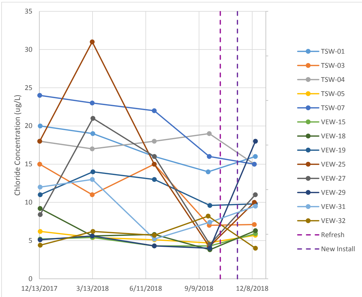
Figure 3.5 Changes in Chloride Concentrations at AOC-65
