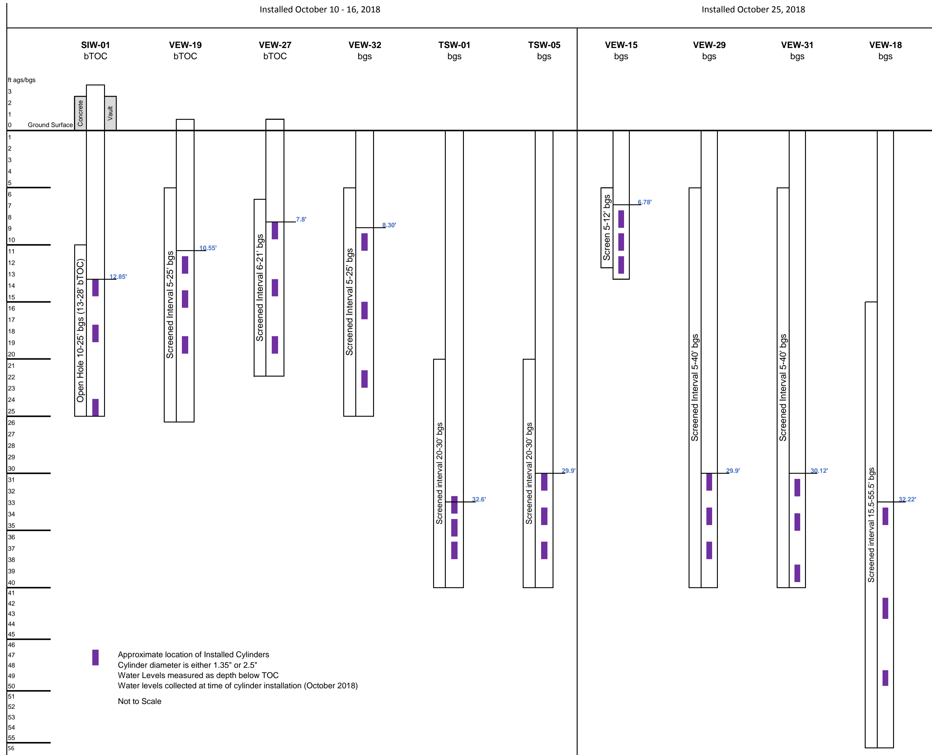
Figure 2.1 2018 Cylinder Distribution at AOC-65 Injection Wells
