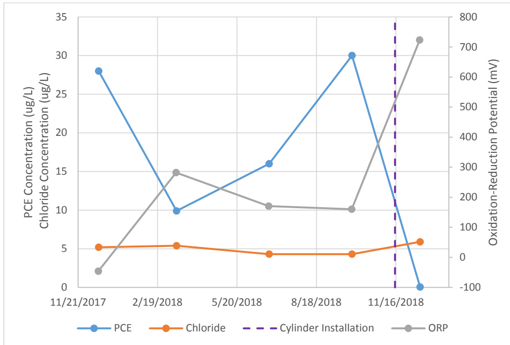
Figure 3.1 Changes in PCE and Chloride Concentrations and ORP Response at VEW-15
