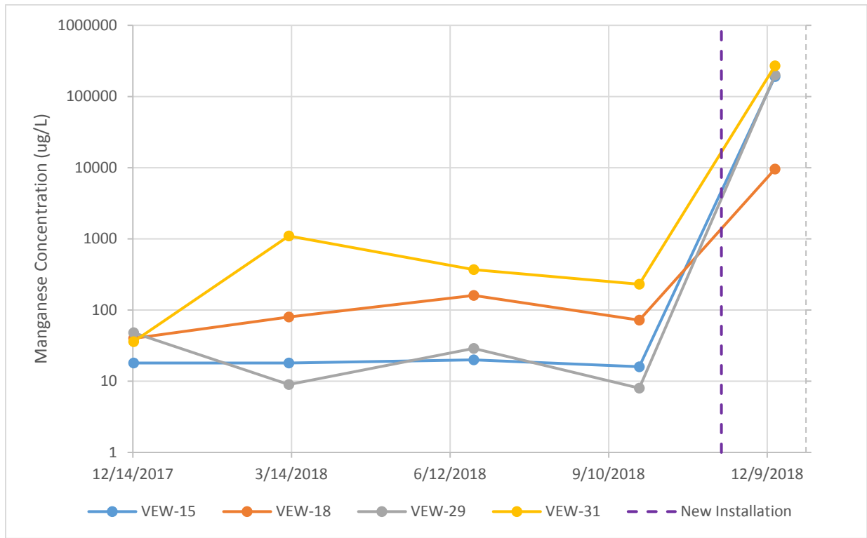
Figure 3.4 Changes in Manganese Concentrations at New ISCO Wells at AOC-65
